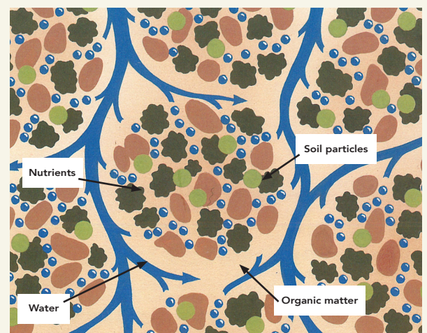
Figure 2: Water moves through the macropores. Water and nutrients are stored within the micropores.
